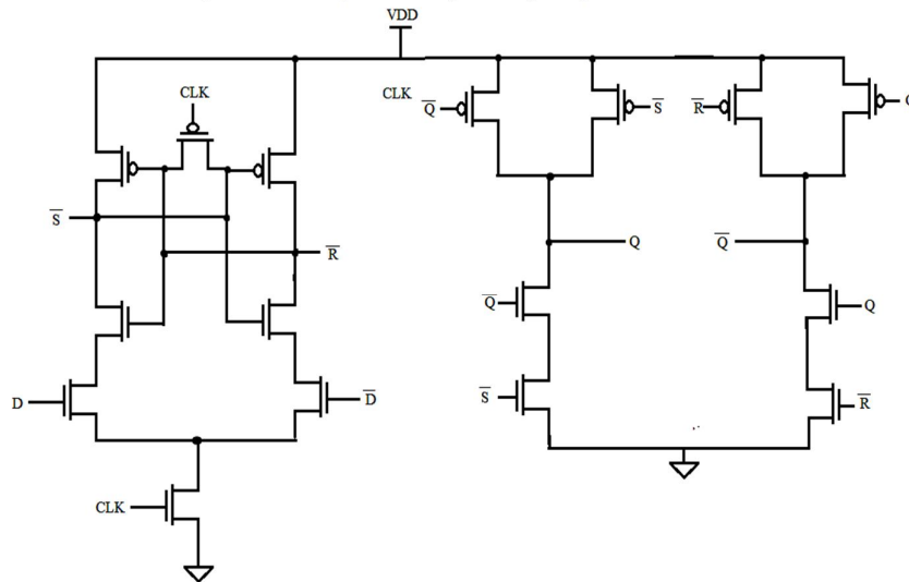
Fig. 8: Circuit diagram of Simplified Sampler
