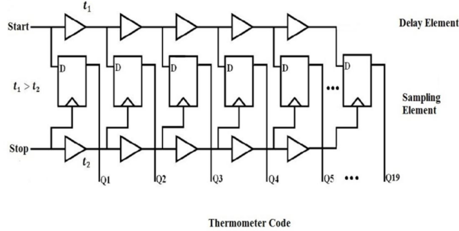
Fig. 2: Vernier Delay Line TDC Architecture [9]
