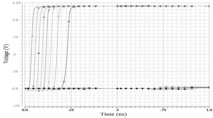
Fig. 15: Output of VDL TDC using Simplified Sampler for delay difference of 0 ps between start and stop signal
