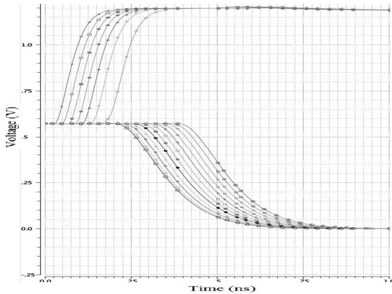
Fig. 9: Output of VDL TDC using Symmetric SR Latch for delay difference of 0 ps between start and stop signal
