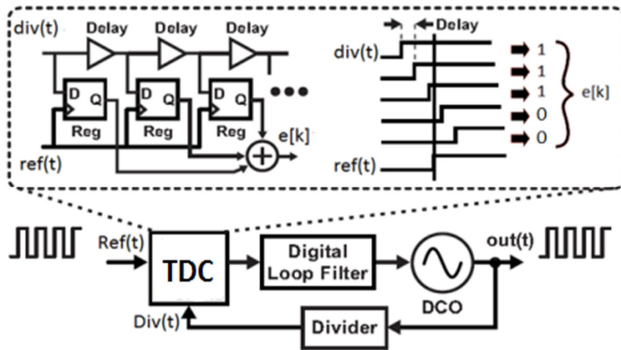
Fig. 1: TDC in All Digital Phase Locked Loop [9]
