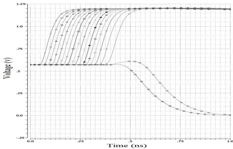
Fig. 10: Output of VDL TDC using Symmetric SR Latch for delay difference of 20 ps between start and stop signal
