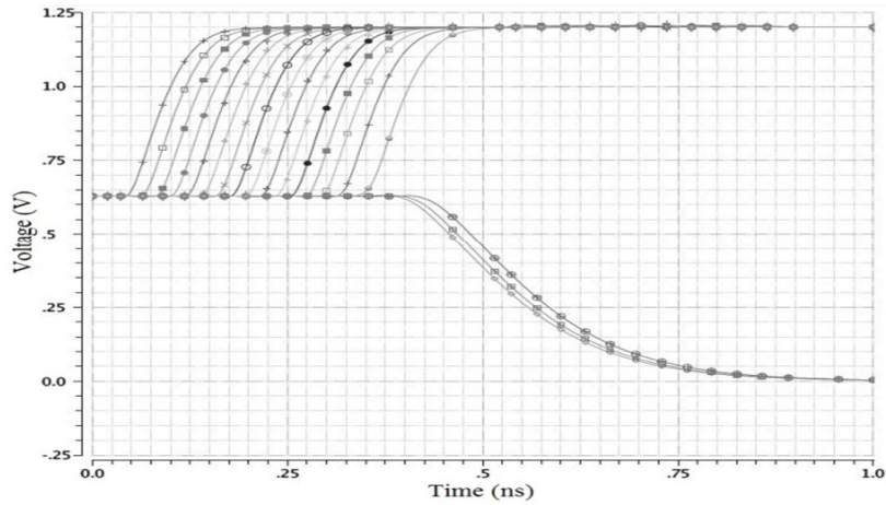
Fig. 13: Output of VDL TDC using Simplified SR Latch for delay difference of 20 ps between start and stop signal
