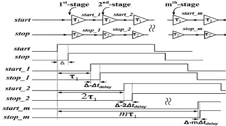
Fig. 3: Signal propagation in a VDL TDC [6]
