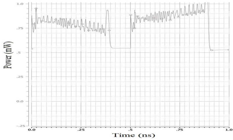
Fig. 11: Plot of Power vs Time for VDL TDC using Symmetric SR Latch
