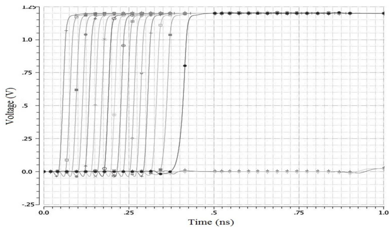
Fig. 16: Output of VDL TDC using Simplified Sampler for delay difference of 20 ps between start and stop signal
