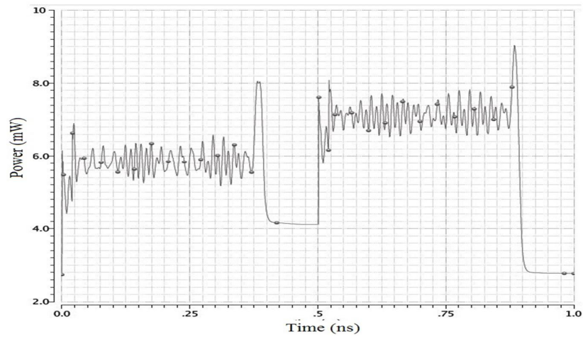
Fig. 14: Plot of Power vs Time for VDL TDC using Simplified SR Latch
