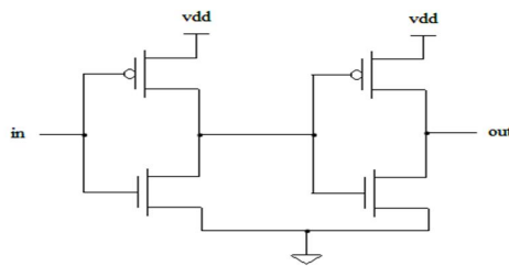
Fig. 4: Circuit diagram of Delay Element
