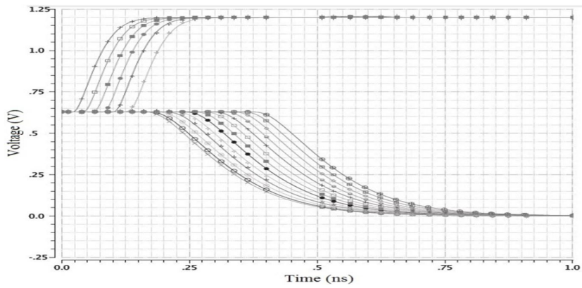
Fig. 12: Output of VDL TDC using Simplified SR Latch for delay difference of 0 ps between start and stop signal
